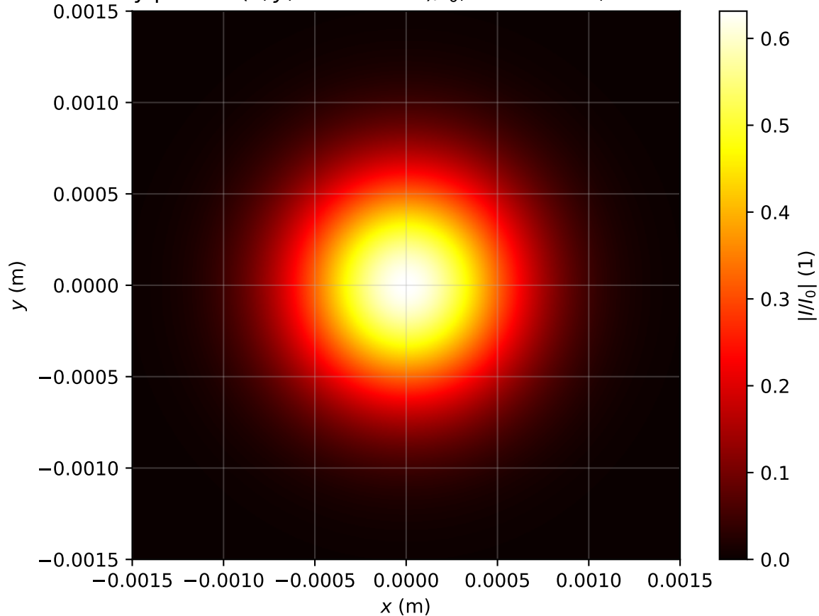
Intensity profile I(x, y, z = 1.672m)/I_0 , Pin=0.1Pcr, artificial time
